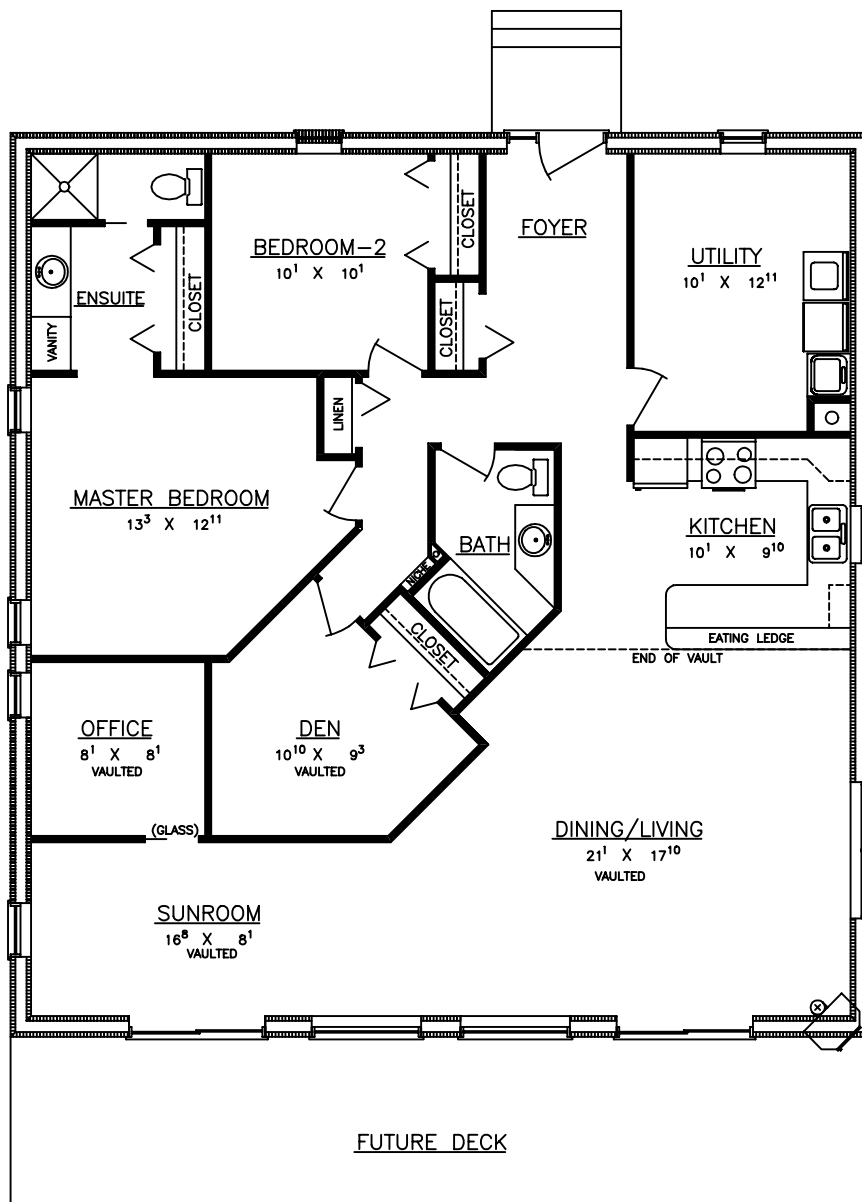
FLOOR PLAN
